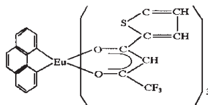
Figure 1. The Structure of \text{Eu}(\text{TTA})_3\text{Phen} .
