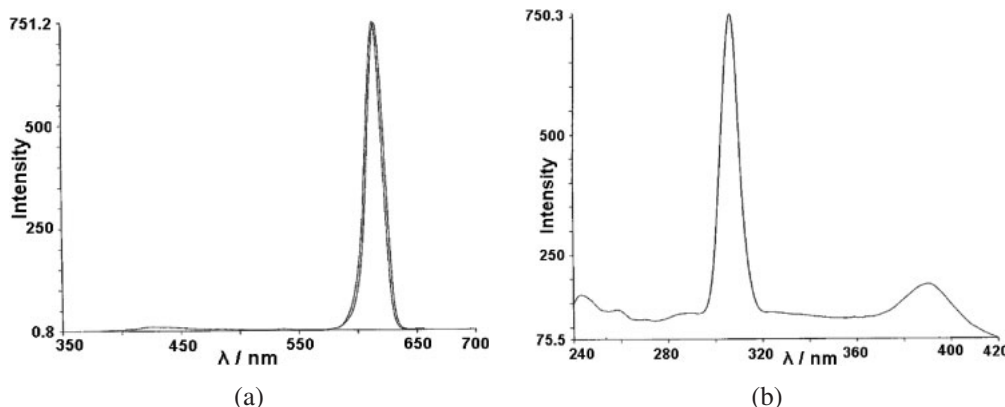
Figure 2. The Emitting spectrum (a) and the Exiting spectrum (b) of \text{Eu}(\text{TTA})_3\text{Phen} .
