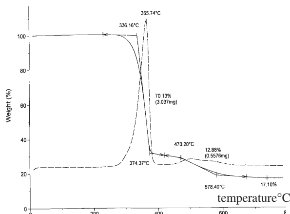
Figure 3. The TGA spectrum of Eu(TTA) 3 Phen.
