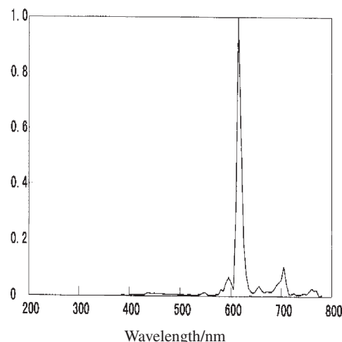
Figure 4. The Emitting spectrum of Eu(TTA) 3 Phen-PC composite material.
