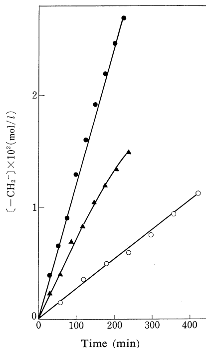
Figure 1. The methylene linkage formed vs. reaction time: ○, Table I exptl no. 4; ●, no. 7; ▲, no. 16.
