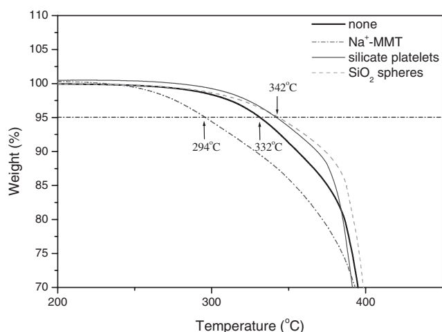
Figure 4. Thermal gravimetric analyses of epoxies with the pristine \text{Na}^+ -MMT, silicate platelets and spheres (1 wt %) at a heating rate of 10^\circ\text{C}/\text{min} in \text{N}_2 .
