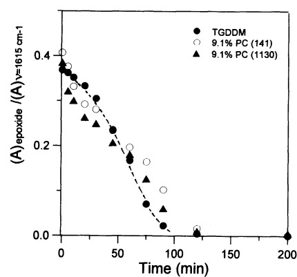
Figure 3. Normalized epoxide FT-IR peak intensity as a function of heating time for (●) TGDDM, (○) TGDDM/PC-141 (9.1 wt%), and (▲) TGDDM/PC-1130 (9.1 wt%).
