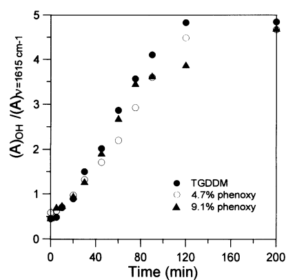
Figure 6. Plots of normalized IR peak intensity of hydroxyl group as a function of heating time for (●) TGDDM, (○) TGDDM/phenoxy (4.7 wt%), and (▲) TGDDM/phenoxy (9.1 wt%).
