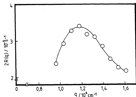
Figure 5. Wavenumber q dependence of the growth rate R(q) in V-BR (70.4)/Gumrosin X (50/50) mixture at 100°C. The peak indicates existence of the maximum growth rate R(q_m) .
