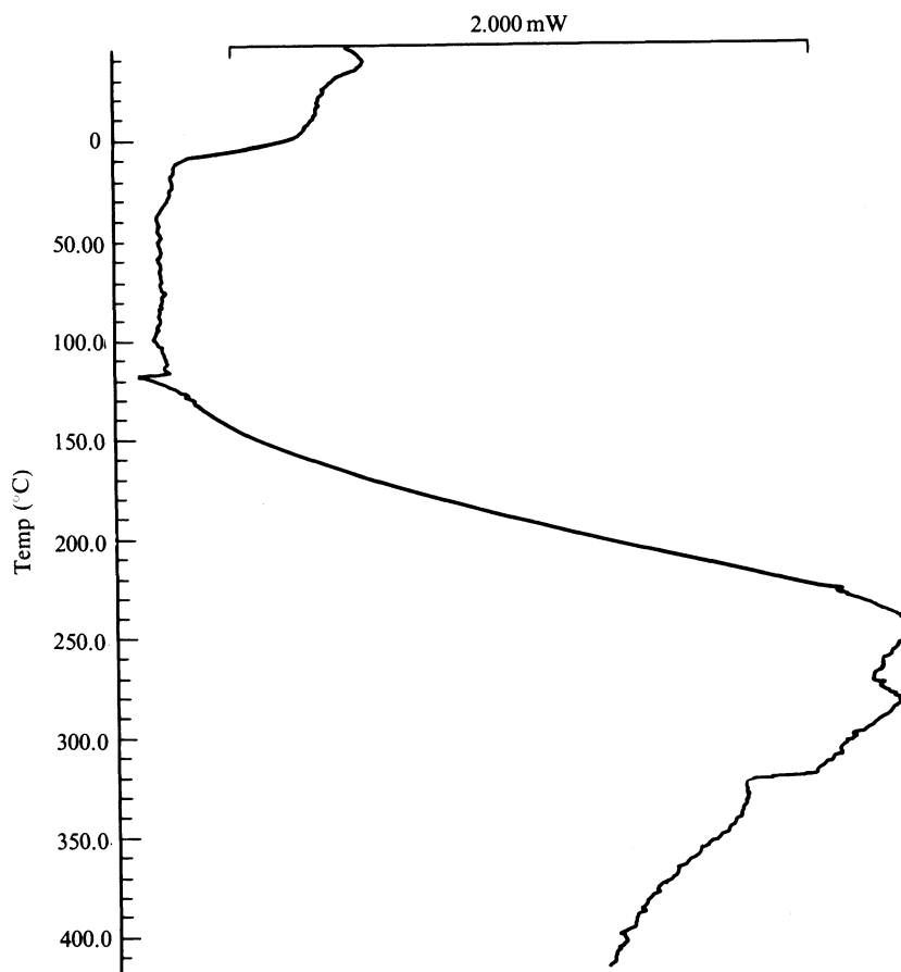
Figure 7. DSC curve of Fe 70003: Heating rate, 10^{\circ}\text{C min}^{-1} .
