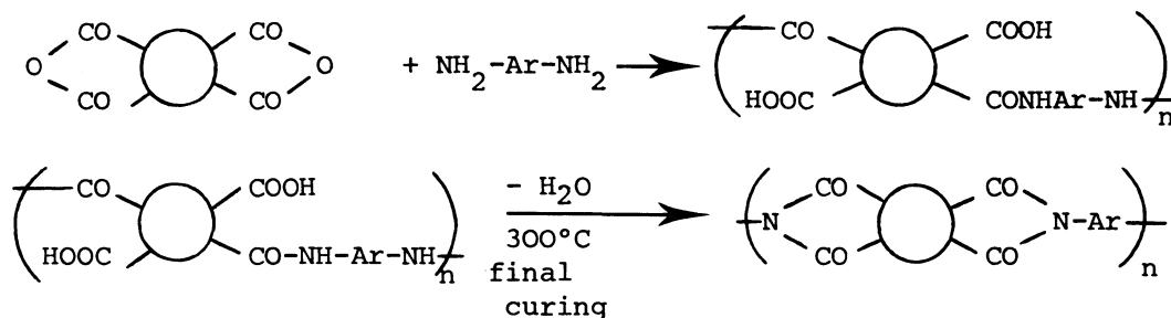
Figure 1. Chemistry of condensation type polyimides.
