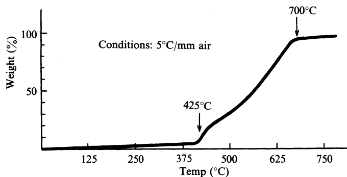
Figure 10. Thermogravimetric analysis. of Fe 70003.
