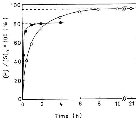
Figure 3. Time-conversion curves on the decarboxylation of S catalyzed by cross-linked polymer catalysts, I-1: [S]_0 , 6 \times 10^{-3} M; pH, 9.0; temp, 30^\circ\text{C} ; O, [C]_0/[S]_0 , 5/100; ●, [C]_0/[S]_0 , 20/100.
